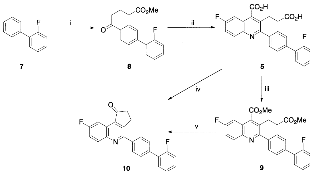
Scheme 4. Reagents: (i) \text{MeO}_2\text{C}(\text{CH}_2)_3\text{COCl} , \text{AlCl}_3 , \text{ClCH}_2\text{CH}_2\text{Cl} , 5^\circ\text{C} , 75%; (ii) 3 , \text{KOH} , \text{EtOH} , dioxane, \text{H}_2\text{O} , 55^\circ\text{C} , 89%; (iii) \text{SOCl}_2 , DMF, toluene, 50^\circ\text{C} , then \text{MeOH} , \text{Et}_3\text{N} , 46%; (iv) \text{TfOH} , 60^\circ\text{C} , 71%; (v) \text{TfOH} , 70^\circ\text{C} , 65%.
