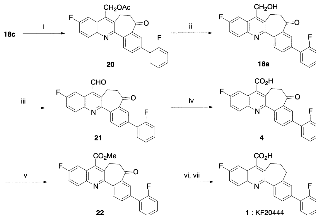
Scheme 9. Reagents: (i) AcONa, AcOH, 110 °C; (ii) aq NaOH, MeOH, rt, 97% from 18c ; (iii) Ac 2 O, DMSO, rt, 90%; (iv) 87% NaClO 2 , NaH 2 PO 4 , DMSO, H 2 O, rt, 98%; (v) MeI, K 2 CO 3 , acetone, 45 °C, 77%; (vi) NaBH 4 , MeOH, rt; (vii) 57% HI, Ac 2 O, AcOH, 110 °C, 73% from 21 .
