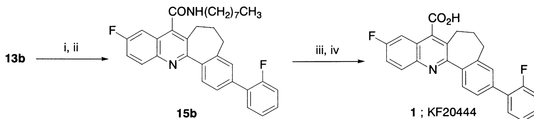
Scheme 6. Reagent: (i) NaBH, MeOH, 5^\circ C ; (ii) 57% HI, Ac_2O , AcOH, 100^\circ C , 96%; (iii) NaNO_2 , Ac_2O , AcOH, rt; (iv) KOH, EtOH, 80^\circ C , 74%.
