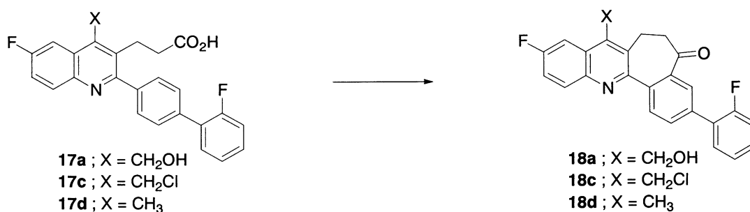
Scheme 7. Reagents: (i) \text{SOCl}_2 , DMF, toluene, 55^\circ\text{C} , then \text{NaBH}_4 , THF, rt, 75%; (ii) \text{MeI} , \text{NaH} , DMF, 5^\circ\text{C} , 94%; (iii) \text{SOCl}_2 , \text{ClCH}_2\text{CH}_2\text{Cl} , rt, 99%; (iv) \text{NaBH}_4 , DMF, rt, 91%; (v) aq \text{NaOH} , \text{MeOH} , 55^\circ\text{C} , 99%; (vi) concd \text{HCl} , \text{AcOH} , 55^\circ\text{C} , 98%.
