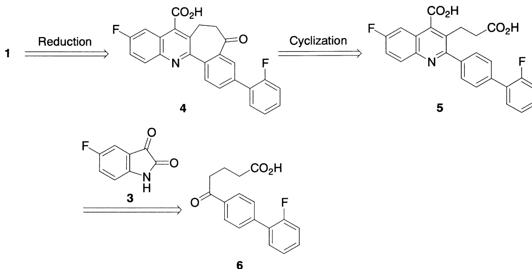
Scheme 3. Synthetic strategy of KF20444.
