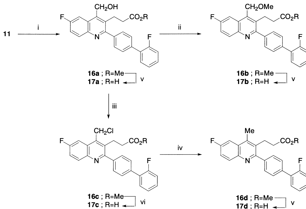
Scheme 7. Reagents: (i) \text{SOCl}_2 , DMF, toluene, 55^\circ\text{C} , then \text{NaBH}_4 , THF, rt, 75%; (ii) \text{MeI} , \text{NaH} , DMF, 5^\circ\text{C} , 94%; (iii) \text{SOCl}_2 , \text{ClCH}_2\text{CH}_2\text{Cl} , rt, 99%; (iv) \text{NaBH}_4 , DMF, rt, 91%; (v) aq \text{NaOH} , \text{MeOH} , 55^\circ\text{C} , 99%; (vi) concd \text{HCl} , \text{AcOH} , 55^\circ\text{C} , 98%.
