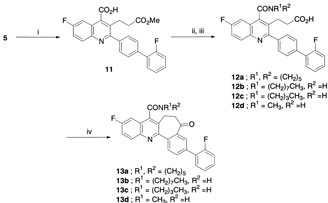
Scheme 5. Reagents: (i) SOCl_2 , toluene, 50^\circ C , then MeOH, 0^\circ C , 99%; (ii) SOCl_2 , DMF, toluene, 60^\circ C , then R^1R^2NH , Et_3N , rt; (iii) aq NaOH, MeOH, 50^\circ C , 43–83%; (iv) (see Table 1).
